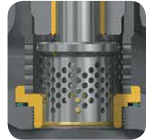
Double-stage trim
