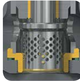
Single-stage trim
