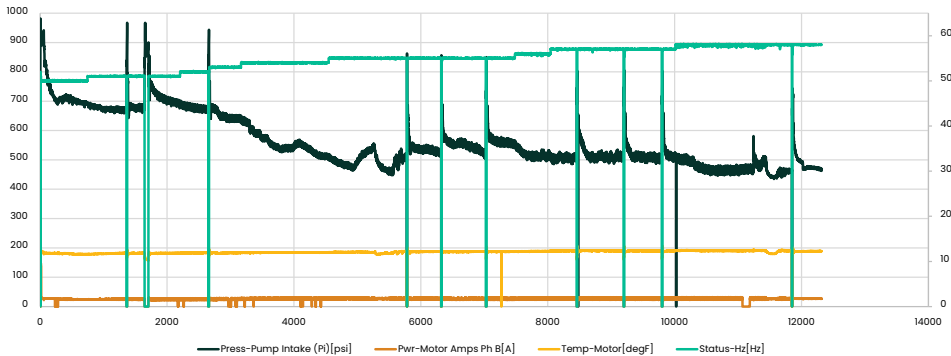
CENesis PHASE solution performance in a well with high gas content in the fluid stream.
