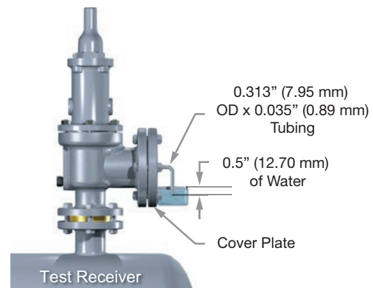
Figure 40: Typical Test Arrangement
