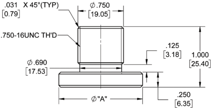
Figure 63: ENERPAC Thread Adaptor
