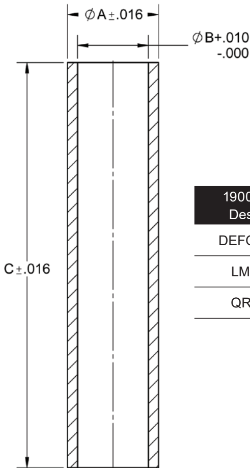
Figure 62: Cylinder
