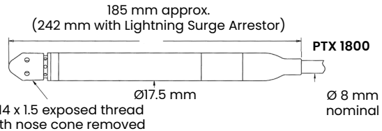
Installation Drawing
