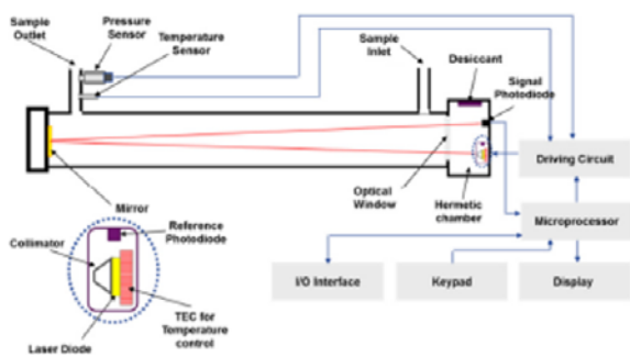
Figure 2: Schematic of TDLAS spectrometer for trace moisture measurement
