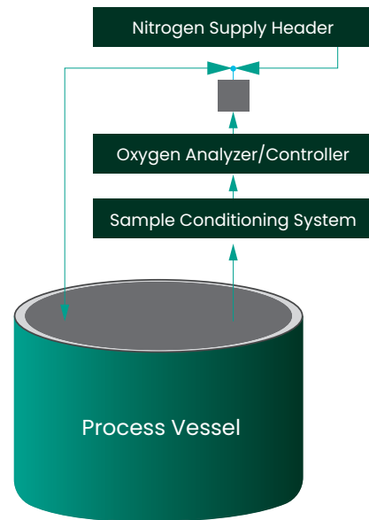
Figure 2: Schematic for tank inerting with O2 analyzer
