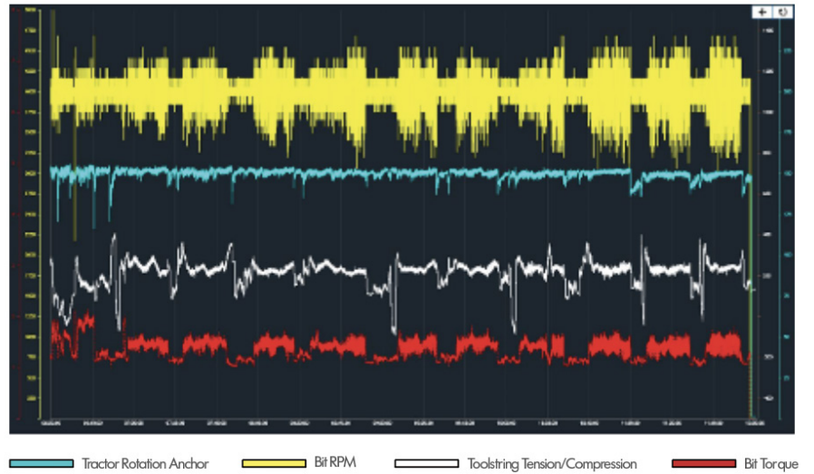
Key milling parameters monitored during the operation
