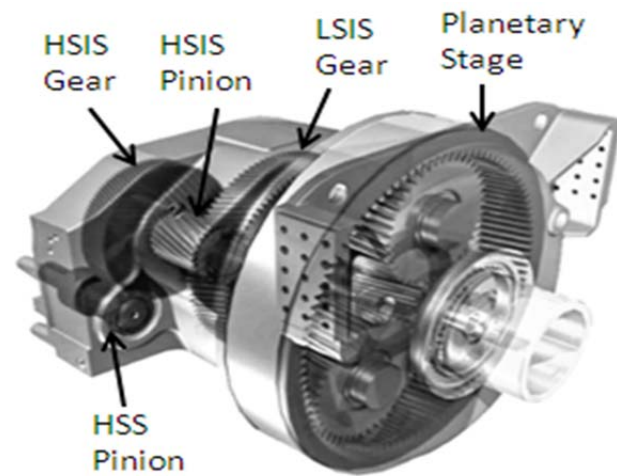
Figure 4: Gearbox Layout
