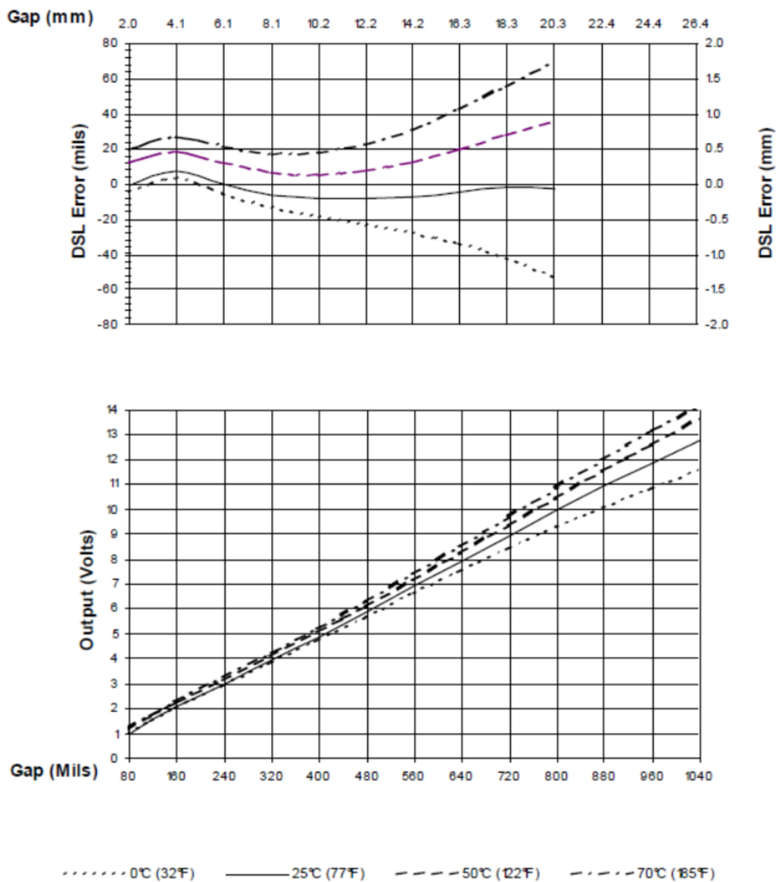
Figure 1: Typical Air Gap 20 mm Proximity Sensor Over Temperature
