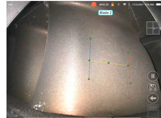
Fig 9c. Blade Counter active showing original tracking region
