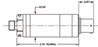
Gauge or sealed gauge/absolute version
