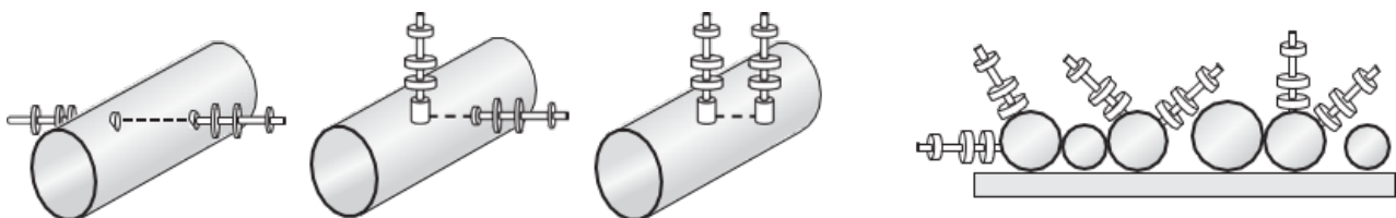
Standard transducer mounting configurations
