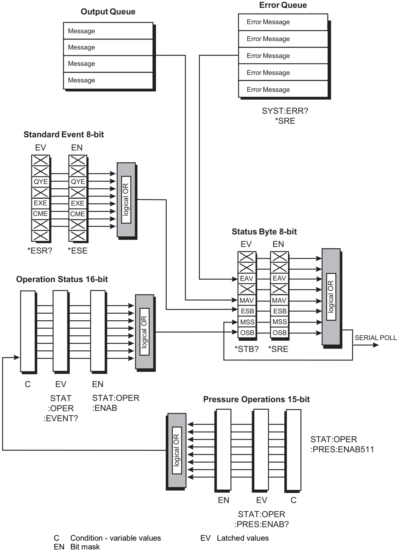
Figure 3-1: Status System
