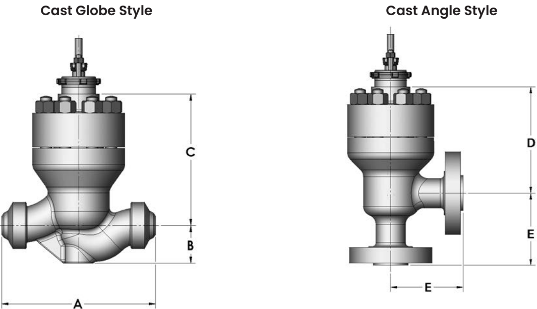
18400/78400 Series Cast Body Dimensions (mm) ASME Class 600 through 2500 and equivalent PN
