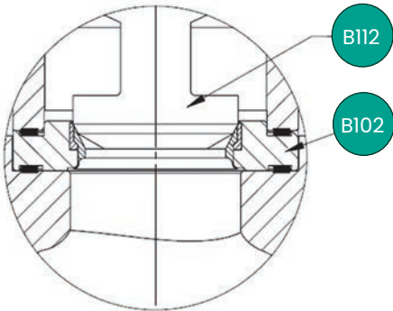
Details Segment for 2" Soft Seat Construction
