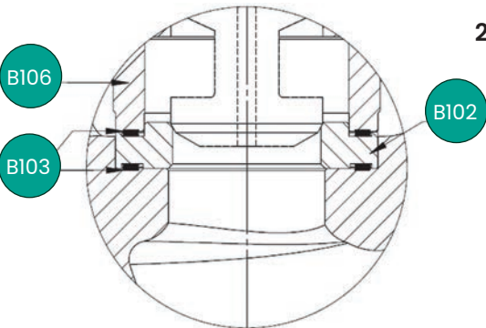
Details Segment for 2" Construction
