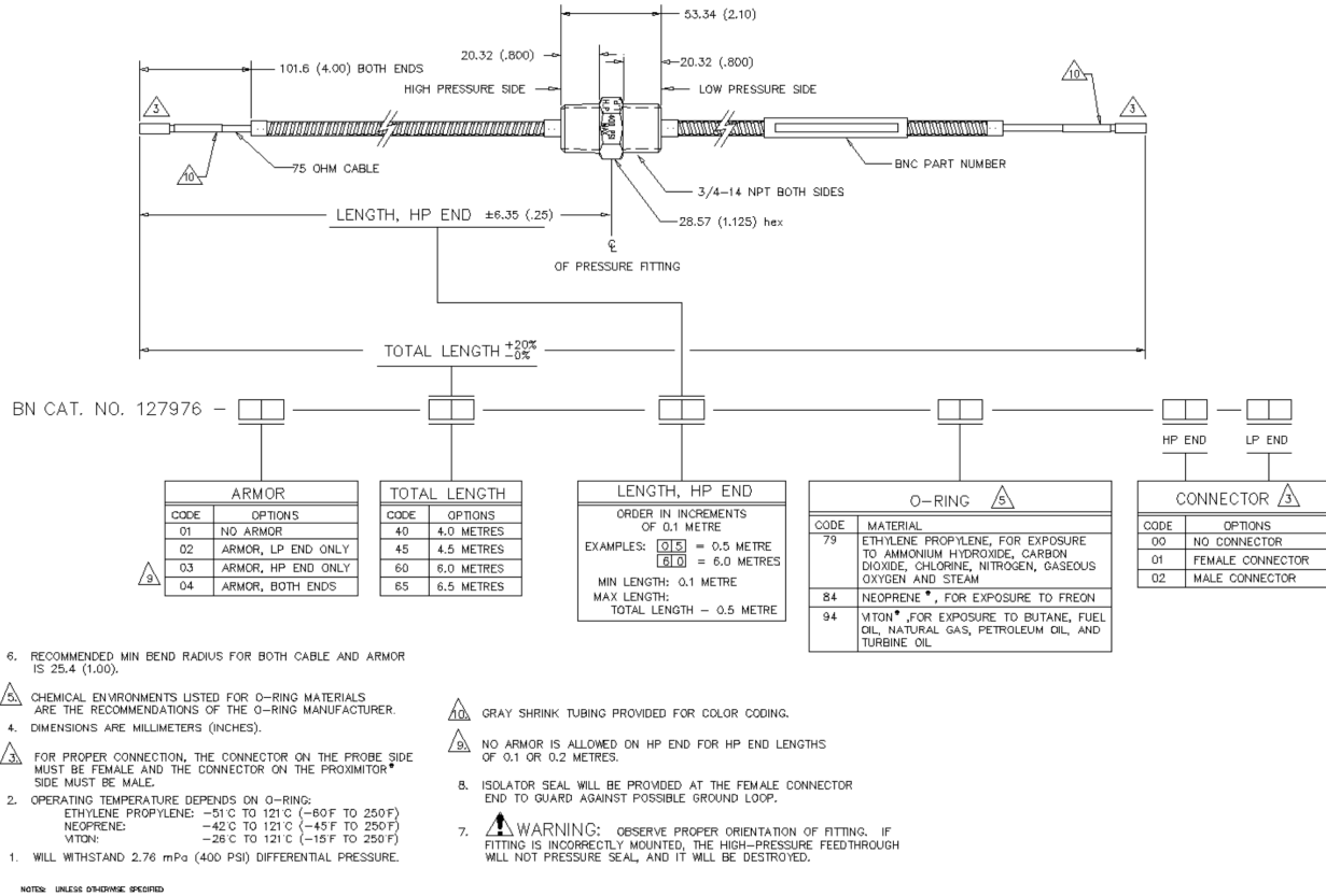
Figure 5: Part Number 127976, High Pressure Feedthrough Single Cable NSv System Dimensions are in millimetres (inches)
