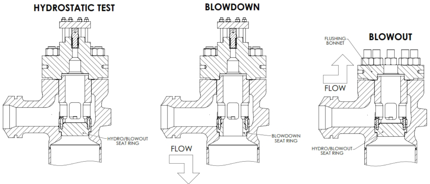
Figure 12: Start-up trim
