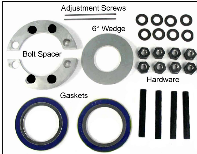
Figure 3: Parts for 150# RF Flange Isolation Valve Installation
