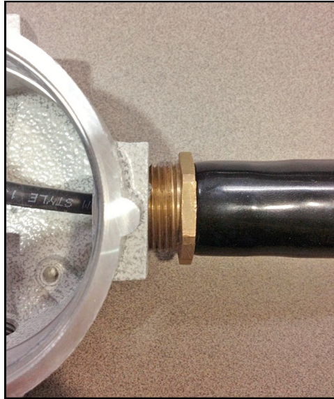
Figure 17: Torquing the Cable Gland
