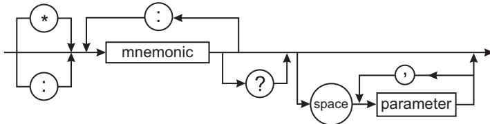
Figure 6-2: Command Syntax
