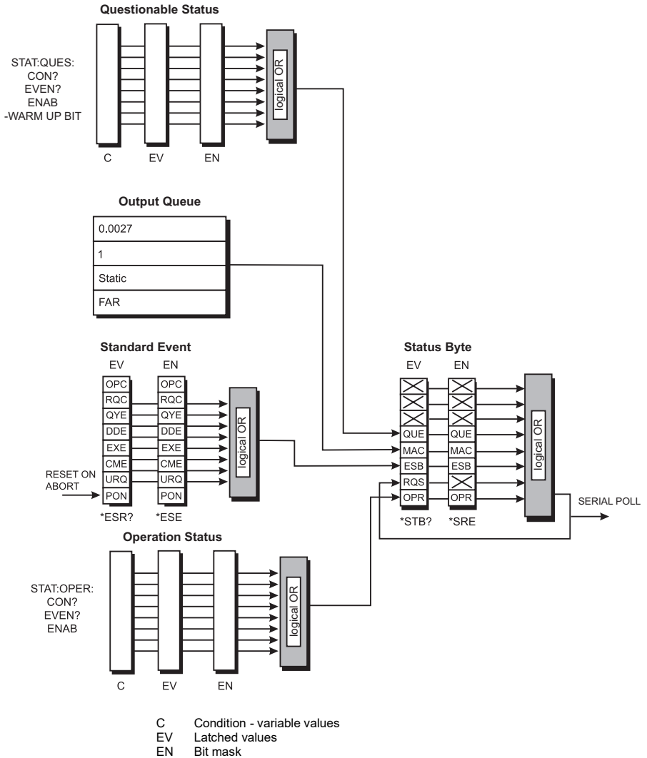
Figure 7-1: Status System
