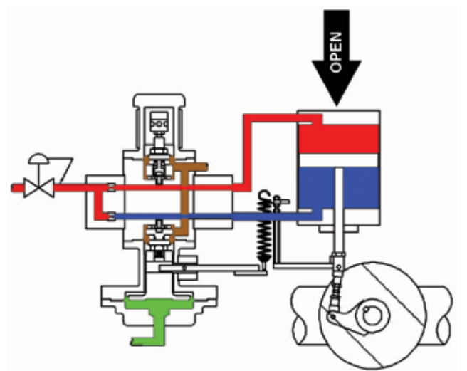
Figure 4.3 - Decrease in Instrument Input Signal to OPEN Valve
