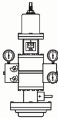
Figure 6.2 - Model HPP-4 Reverse-Acting Positioner (Split Range)
