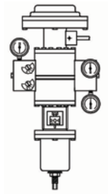
Figure 6.4 - Model HPP-4 Direct-Acting Positioner (Split Range)
