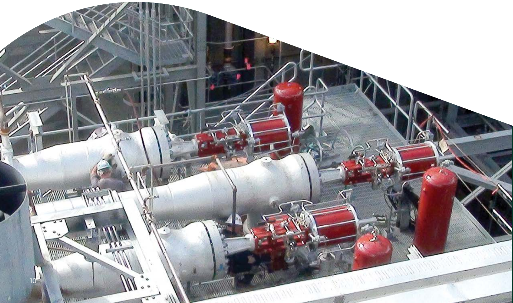
Robust plug design extends service life.
