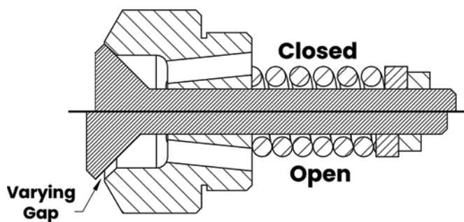
Competitors Nozzle Design
