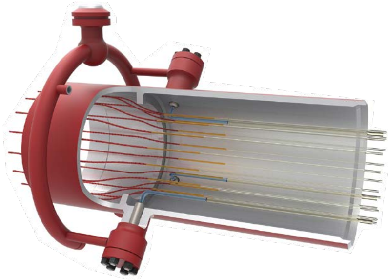
Water Injection with Flow Profiler
