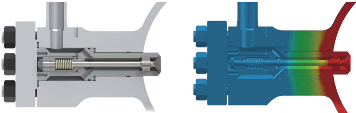
Spring loaded spray nozzles designed to move springs away from high temperature/high cycling areas for extended operating life.
