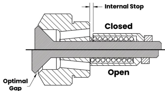
Masoneilan Nozzle Design
