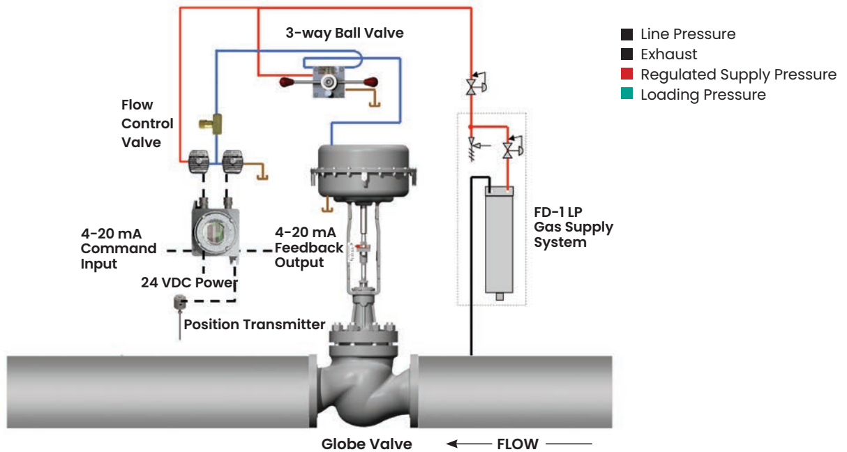
Figure 1 - DNGP Configured with Becker LD Series Actuator and Globe Control Valve
