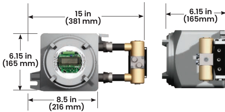
Figure 4 - DNGP with High Pressure 5/3 Solenoid Valve for Standard Double-Acting Application.
