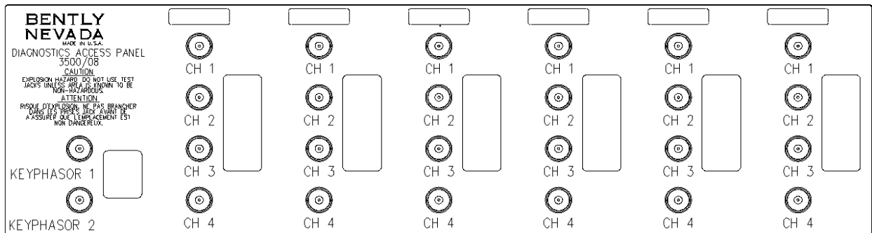
Figure 1: 3500/08 Front View
