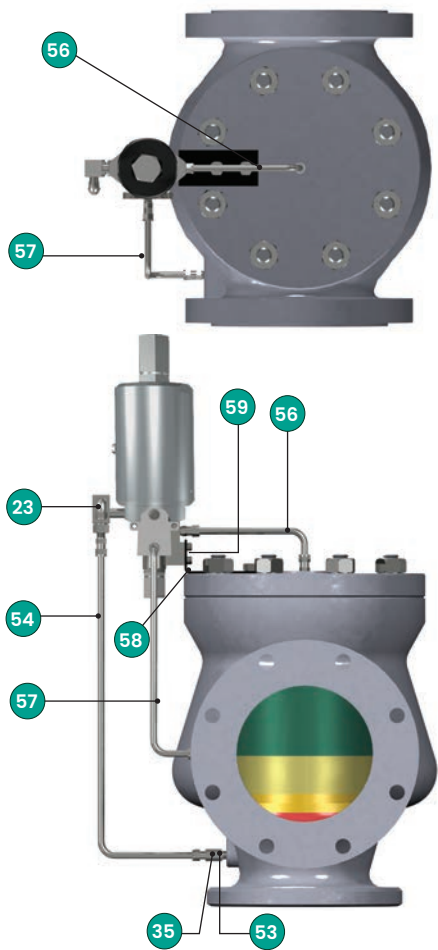
Pilot Valve with Field Test Connection (Standard For All Media Applications)
