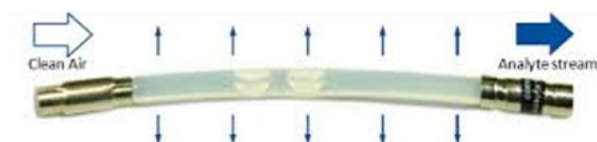
Figure 4. Permeation tubes
