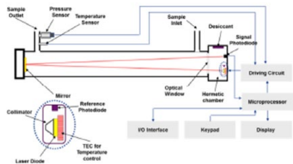
Figure 2. Schematic of TDLAS spectrometer for trace moisture measurement
