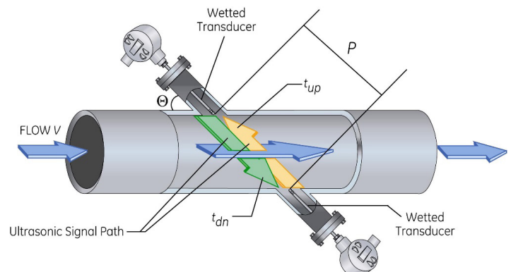
Figure 1. The operating principle of a transit time-based ultrasonic flow meter.
