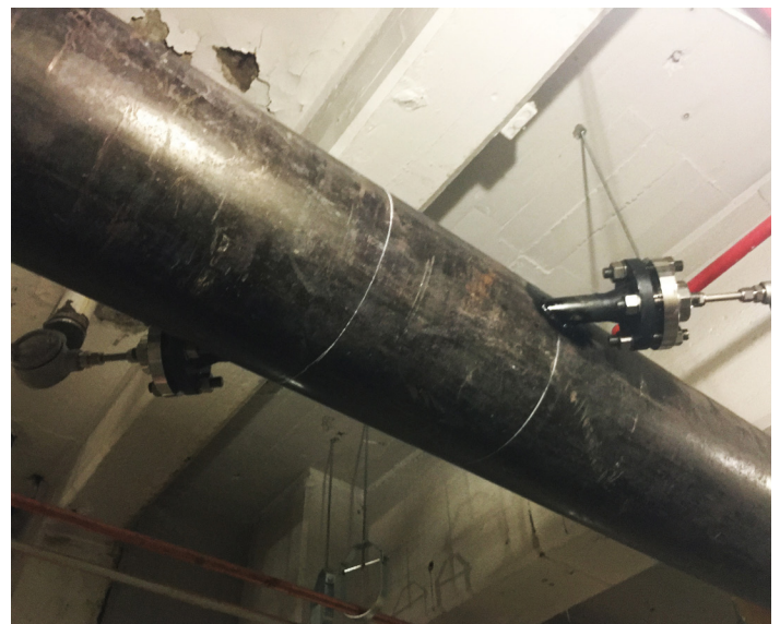
Steam cold tap installation
